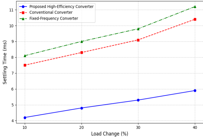
Fig 6: Settling Time Comparison under Load Transient
