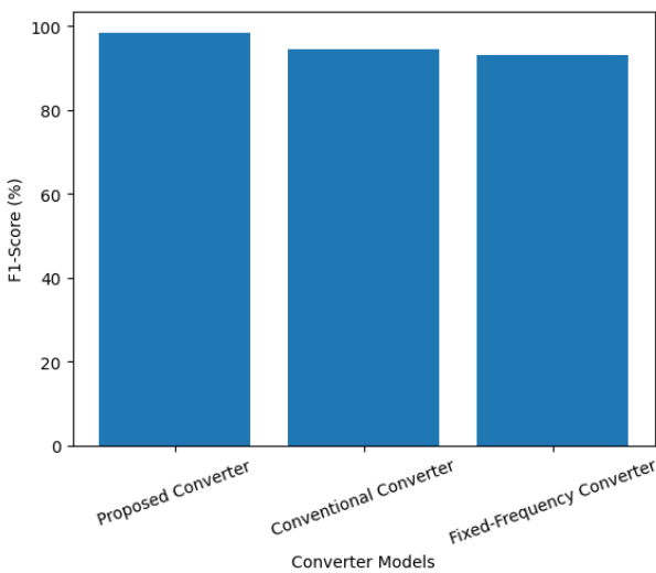
Fig 12: F1-Score Comparison
