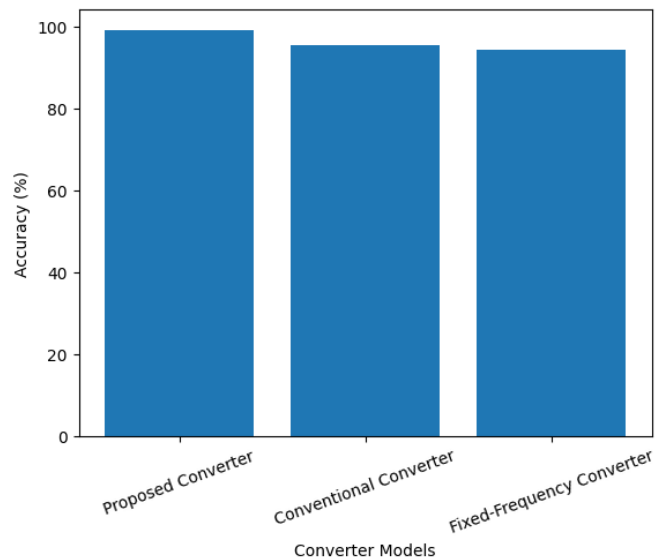
Fig 9: Accuracy Comparison
