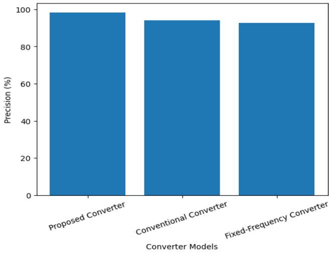
Fig 10: Precision Comparison
