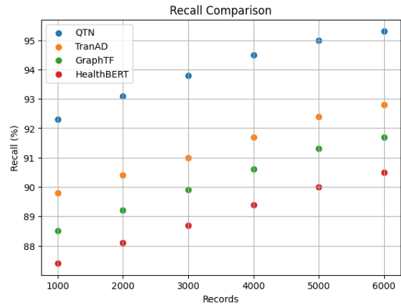
Fig 5: Recall Levels
