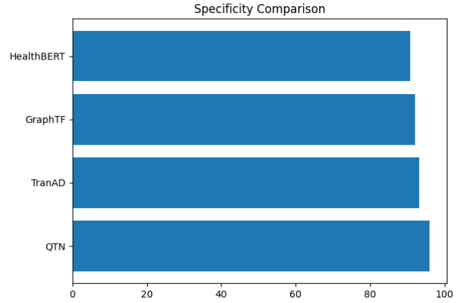
Fig 7: Specificity Levels
