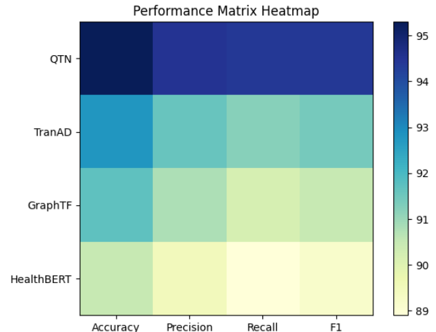
Fig 12: Performance Matrix
