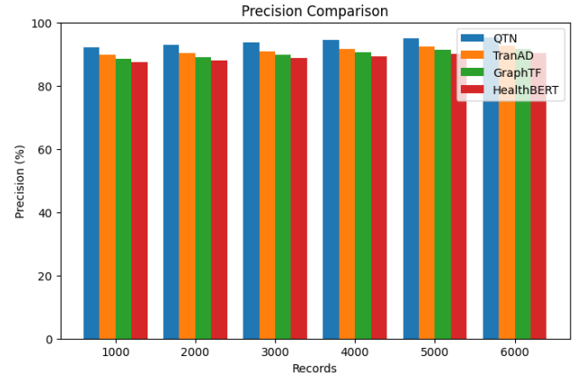
Fig 4: Precision Levels
