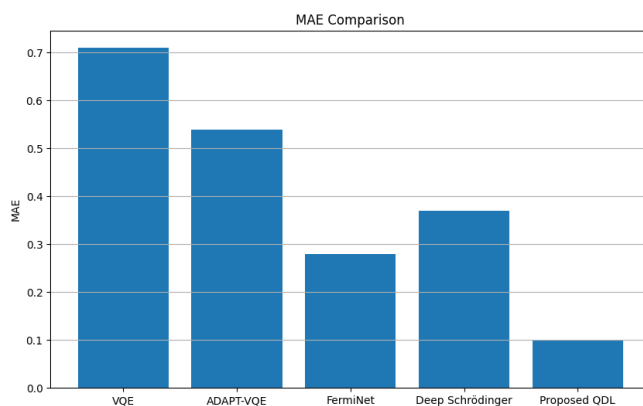
Fig 7: MAE Comparison of Existing and Proposed Approaches
